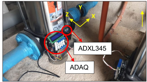
Figure 3. ADAQ installation at the water pump motor showing all axes' direction
